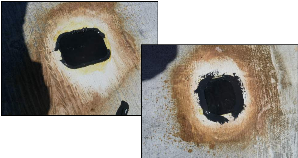
Photos 1 - 2 - Typical roof core repairs
