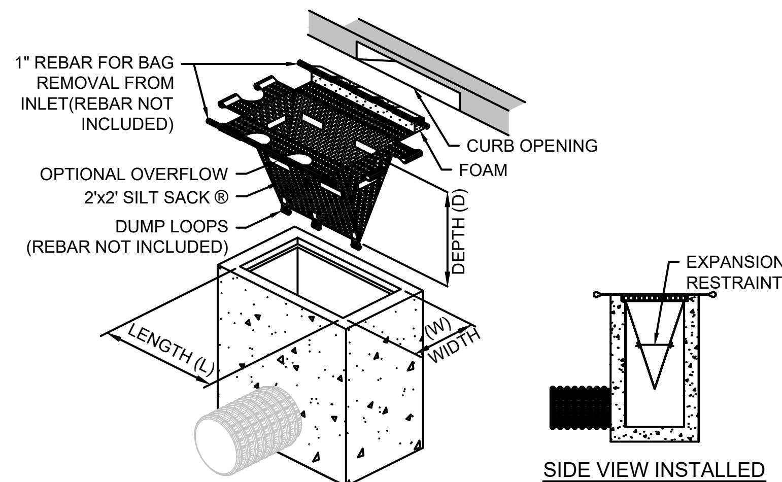
SILT SACK NOT TO SCALE
