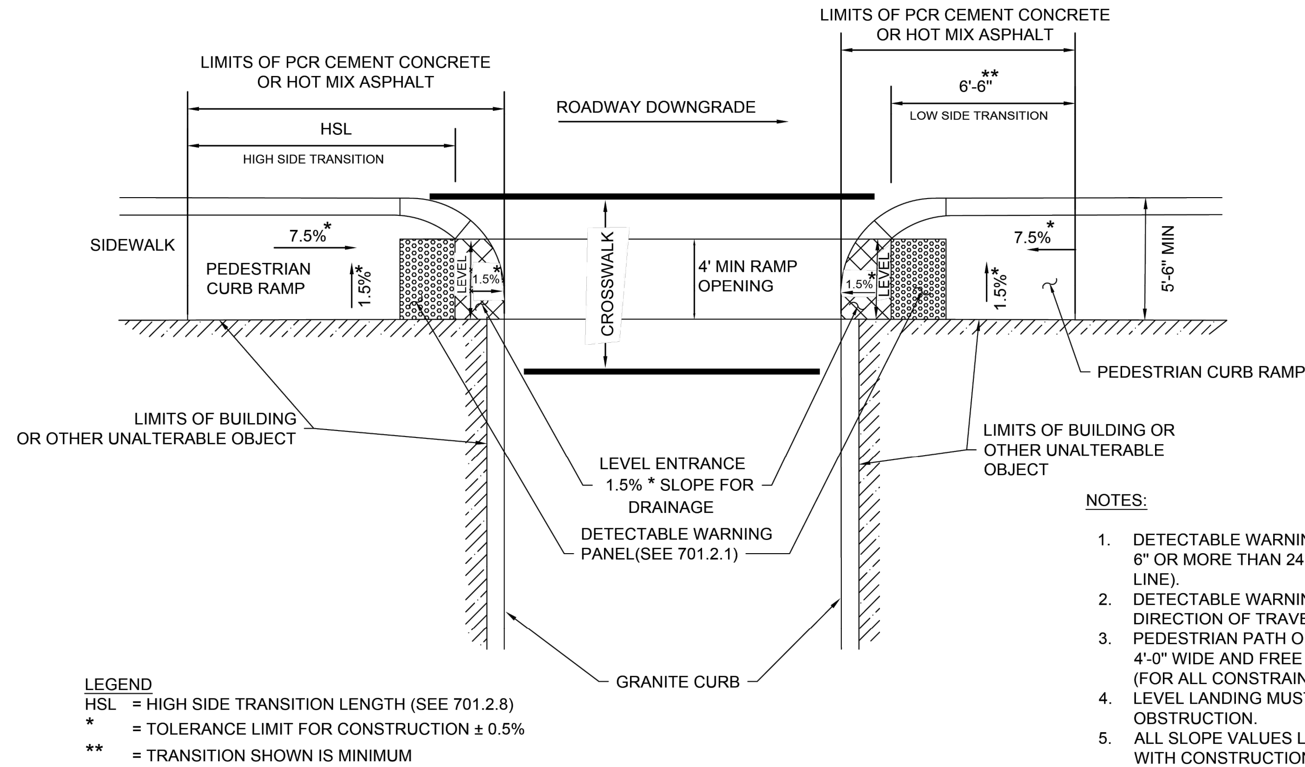
PEDESTRIAN CURB RAMP FOR ONE CONTINUOUS DIRECTION OF PEDESTRIAN TRAVEL (701.2.5) NOT TO SCALE
