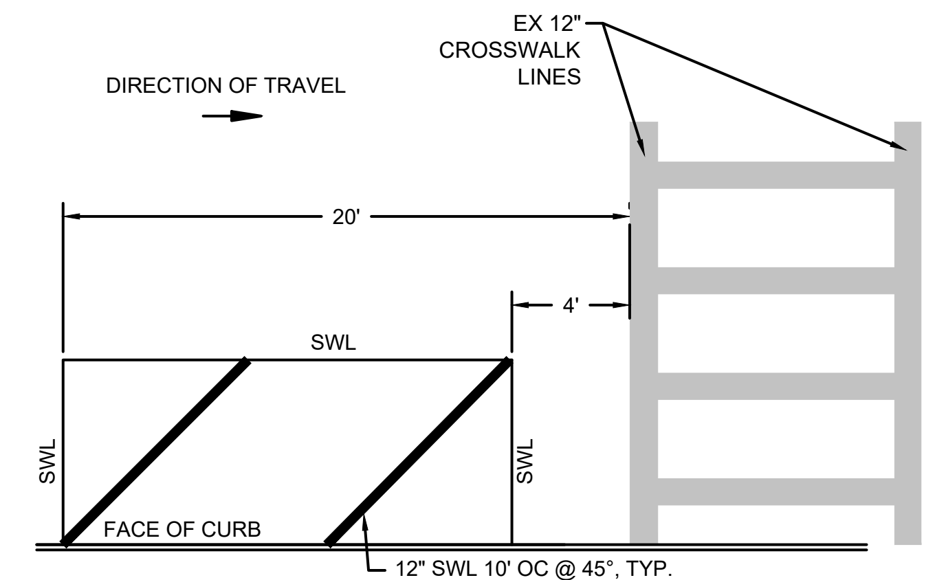
DAYLIGHTING WITHOUT STOP BAR NOT TO SCALE
