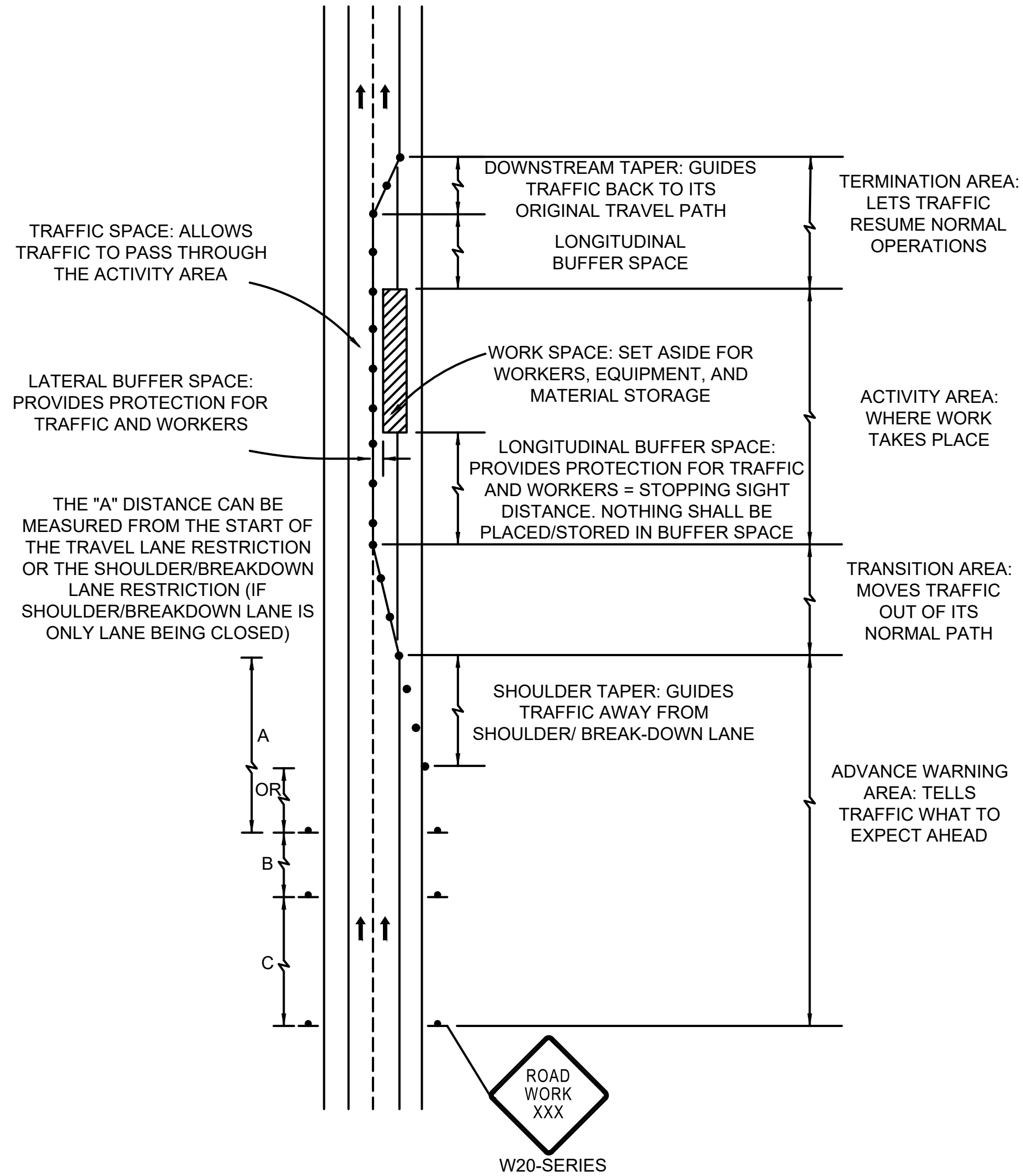
COMPONENT PARTS OF A TEMPORARY TRAFFIC CONTROL (TTC) ZONE NOTE TO SCALE
