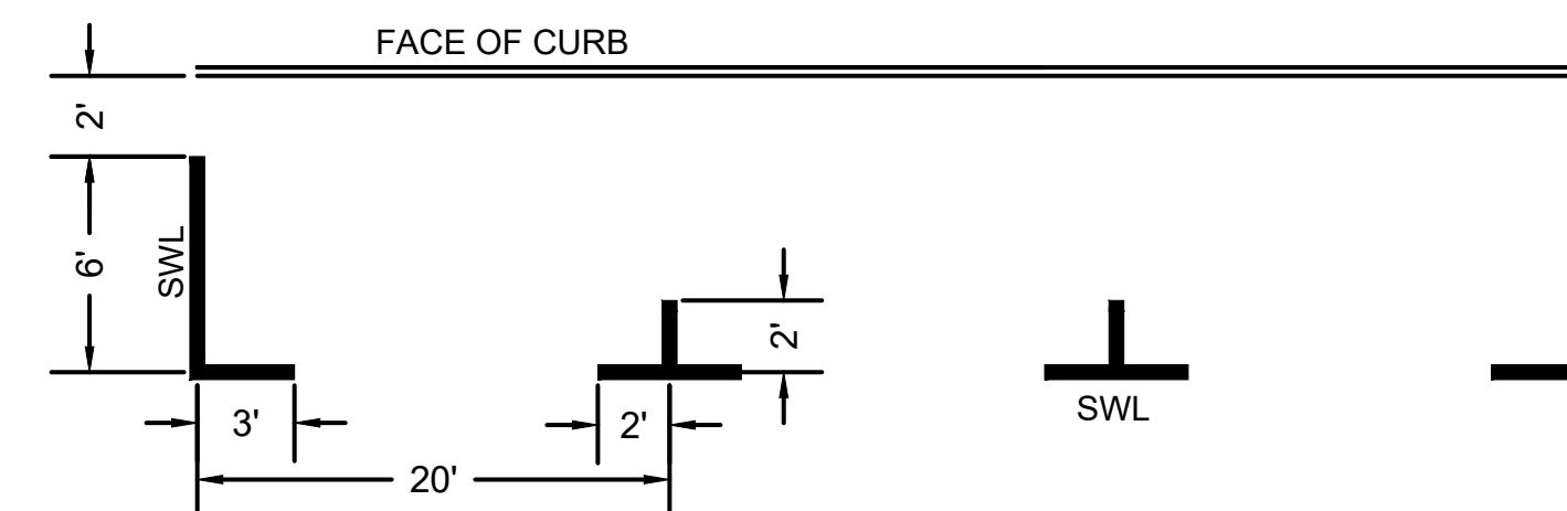
PARKING STALL MARKINGS NOT TO SCALE
